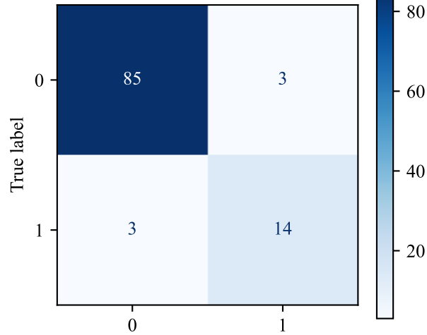
Fold 5
