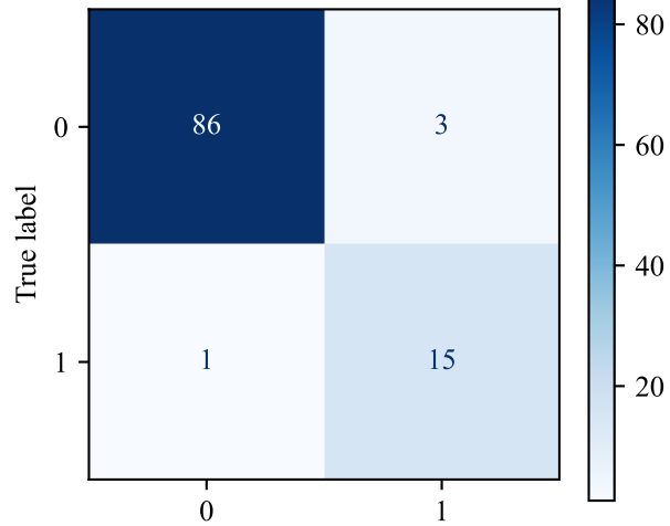
Fold 1
