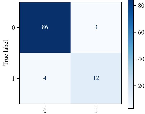
Fold 2
