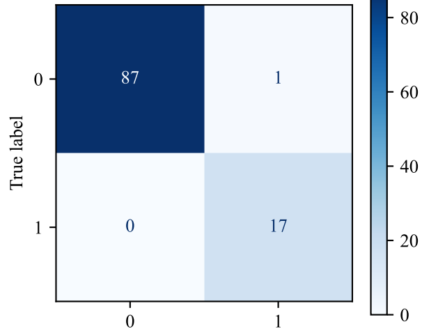
Fold 4
