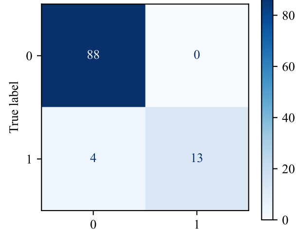
Fold 3
