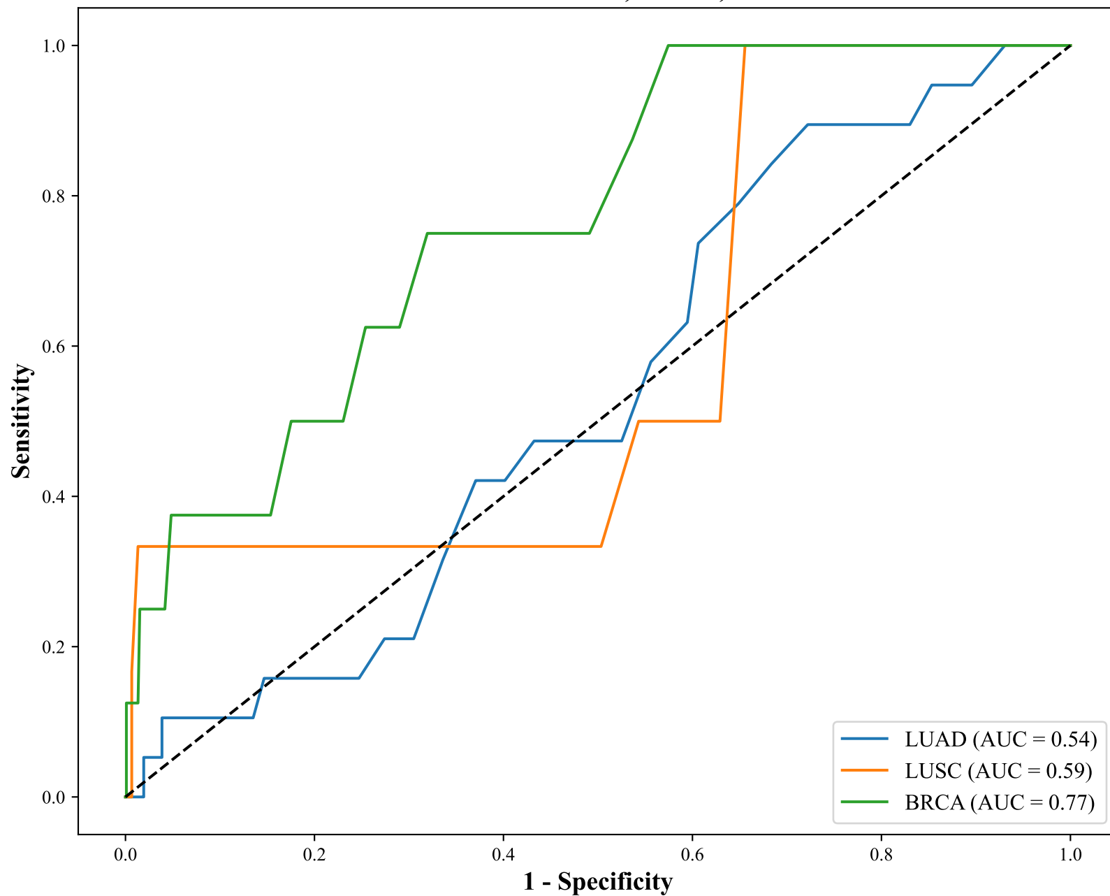
ROC Curves for LUAD, LUSC, and BRCA
