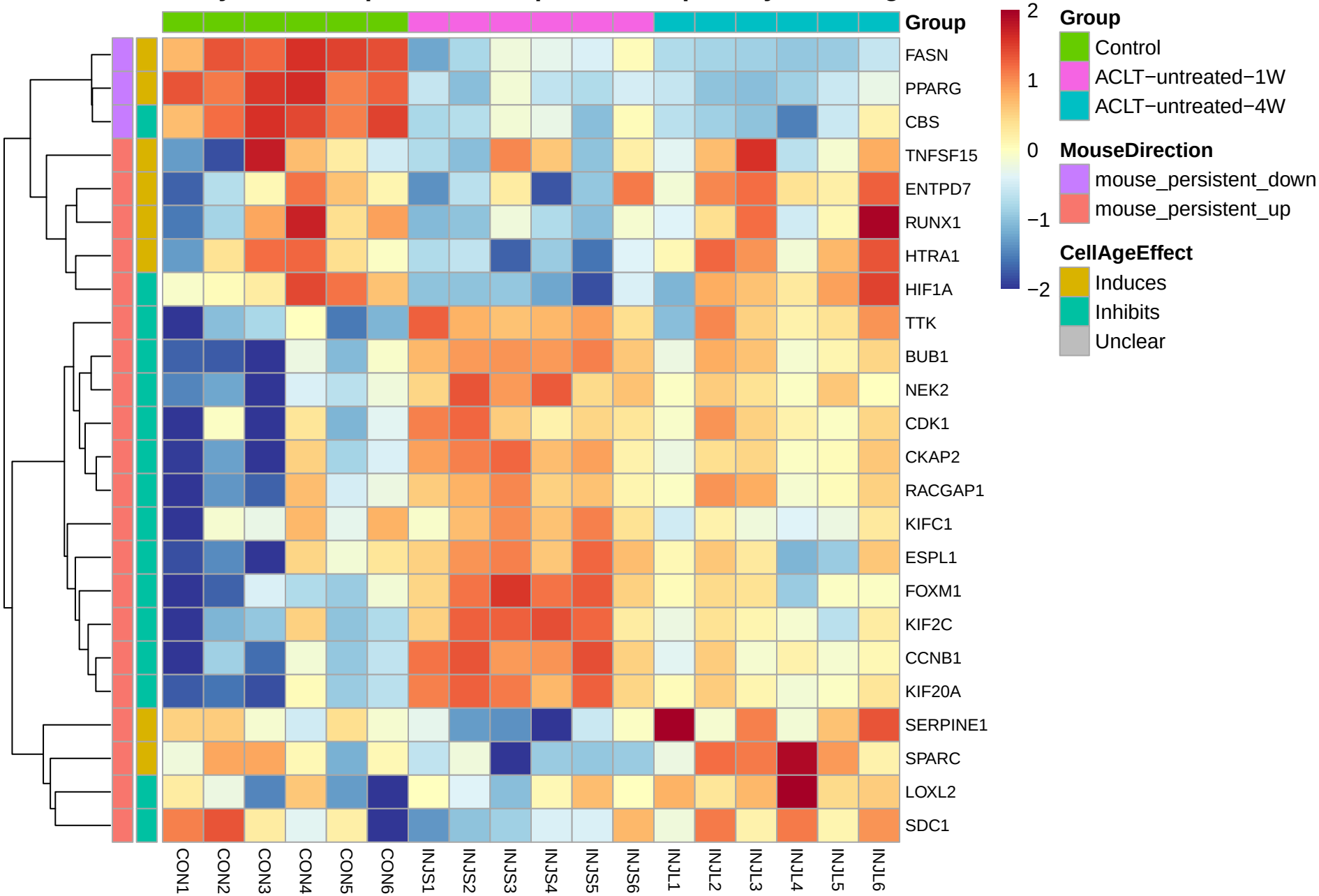
Sensitivity audit: fastp-trimmed expression of primary 24 core genes
