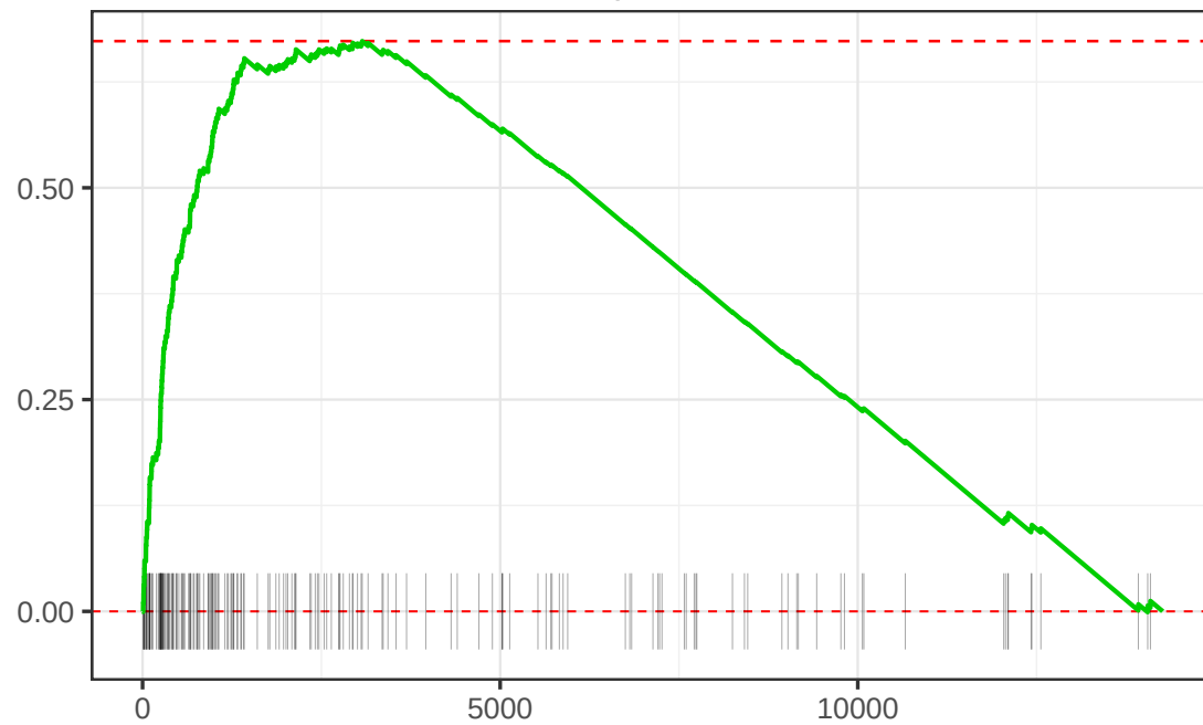
EMT / ECM remodeling — 4W NES = 3.126 | FDR = 7.38e-36
