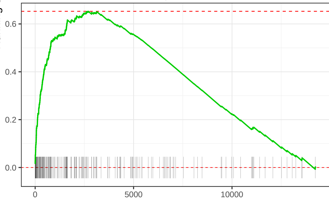
EMT / ECM remodeling — 1W NES = 3.128 | FDR = 7.84e-32
