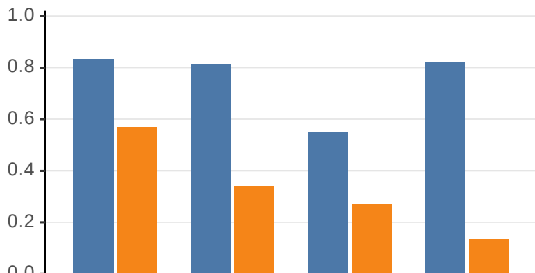
Pearson r
