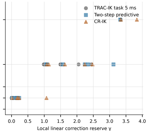
b UR5e: 12 states / 4 trajectories
