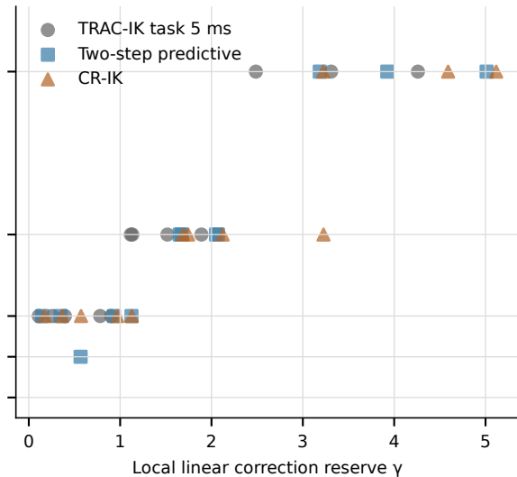
b UR5e: 12 states / 4 trajectories
