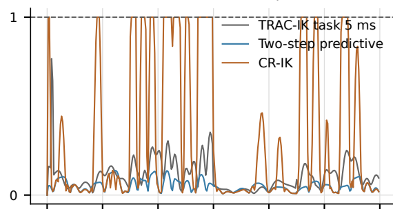
UR5e — fixed first-UID curvature path
