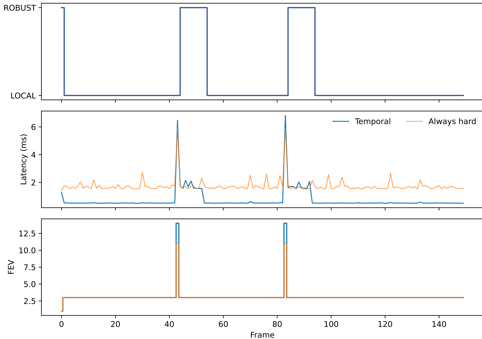
ur5e: representative temporal trajectory
