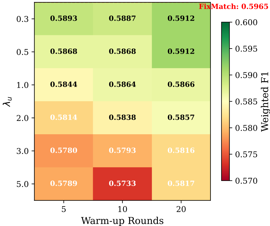
ECR \lambda_u Sensitivity (IEMOCAP 50%)
