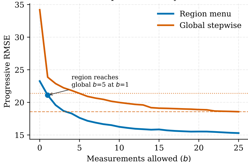
Superconductivity
