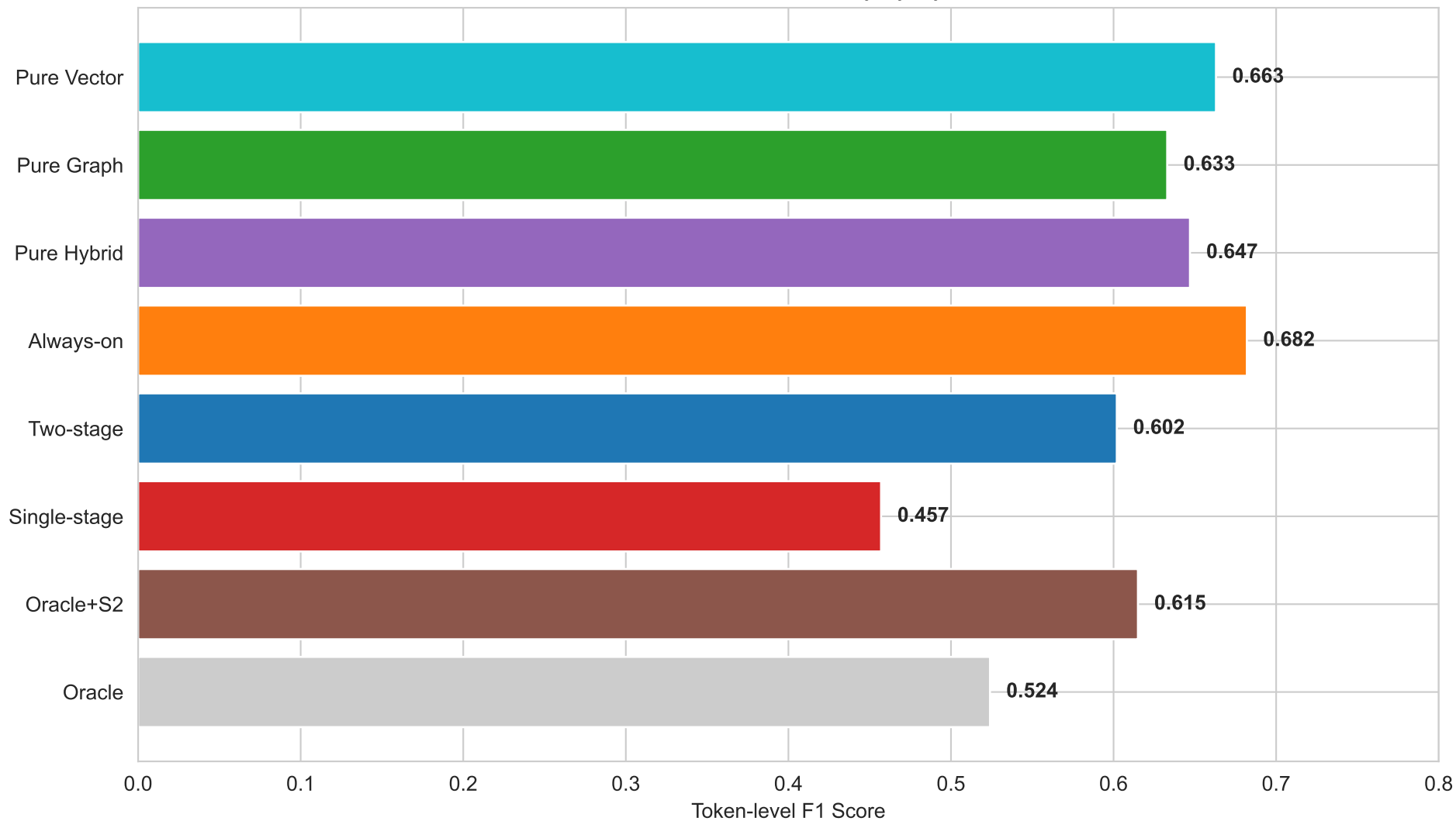
End-to-End Answer Quality by System
