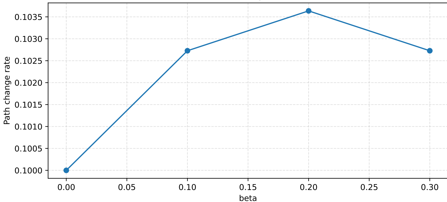
DA-FW: Route Change Rate vs beta
