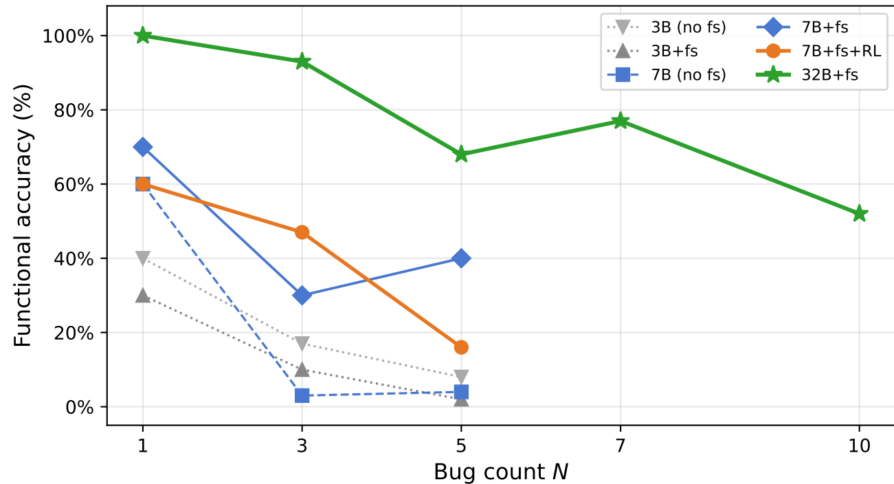
CDBench degradation curves
