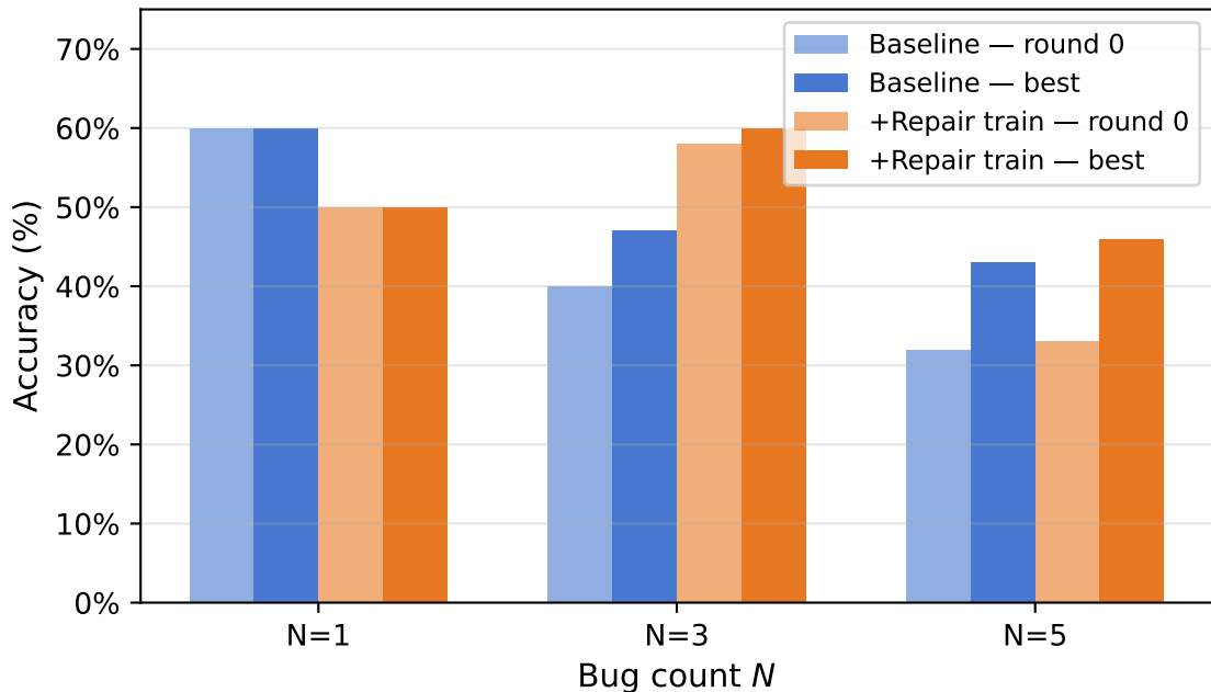
Repair-conditioned GRPO vs. baseline
