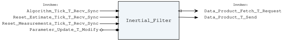
Figure 1: Inertial Filter component diagram.
