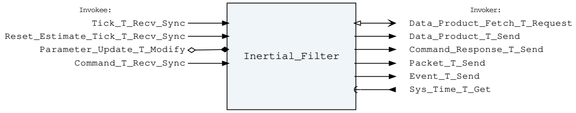
Figure 1: Inertial Filter component diagram.
