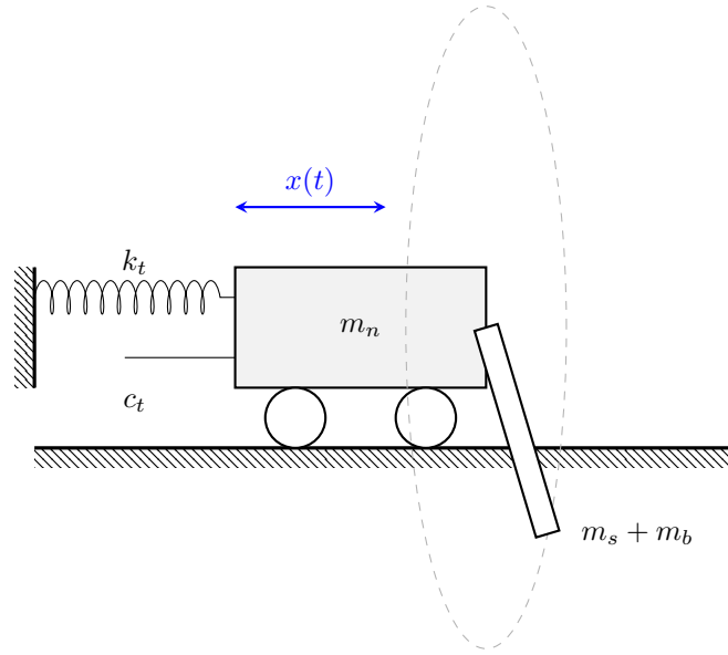
Fig. 8. Refined 2-DOF model with azimuthal rotation ( \psi ).
