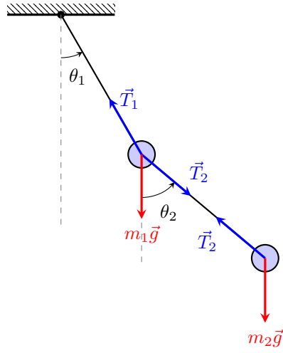
Fig. 7. Free Body Diagram of a double pendulum. The coordinates \theta_1 and \theta_2 are defined relative to the vertical. Mass m_1 is acted upon by gravity m_1\vec{g} and the tensions from both rods, while m_2 is acted upon by m_2\vec{g} and the tension \vec{T}_2 .
