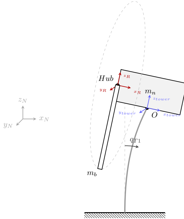
Fig. 10. Schematic of the Flexible Tower model with modal deflection q_{T1} .
