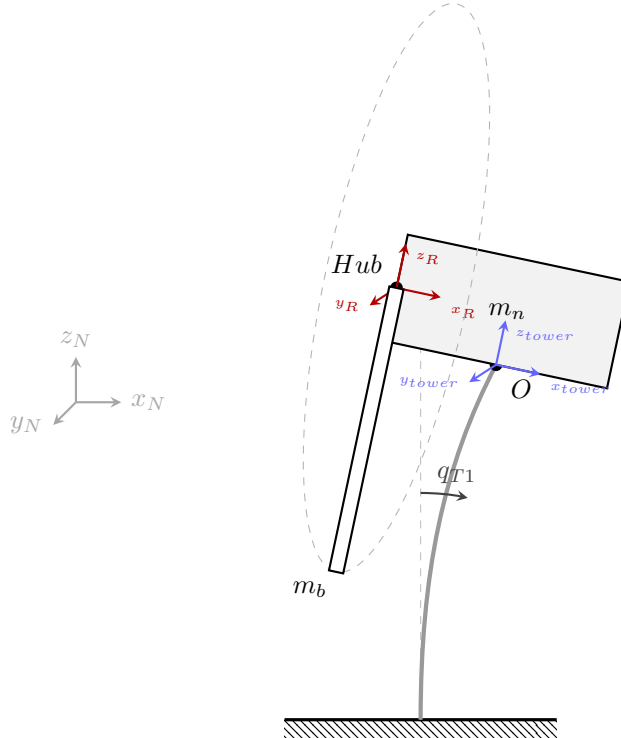
Fig. 7. Schematic of the Flexible Tower model with modal deflection q_{T1} .
