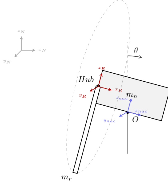
Fig. 1. Schematic of the Tilting Nacelle model showing coordinate frames and mass positions.
