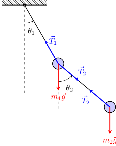
Fig. 4. Free Body Diagram of a double pendulum. The coordinates \theta_1 and \theta_2 are defined relative to the vertical. Mass m_1 is acted upon by gravity m_1\vec{g} and the tensions from both rods, while m_2 is acted upon by m_2\vec{g} and the tension \vec{T}_2 .
