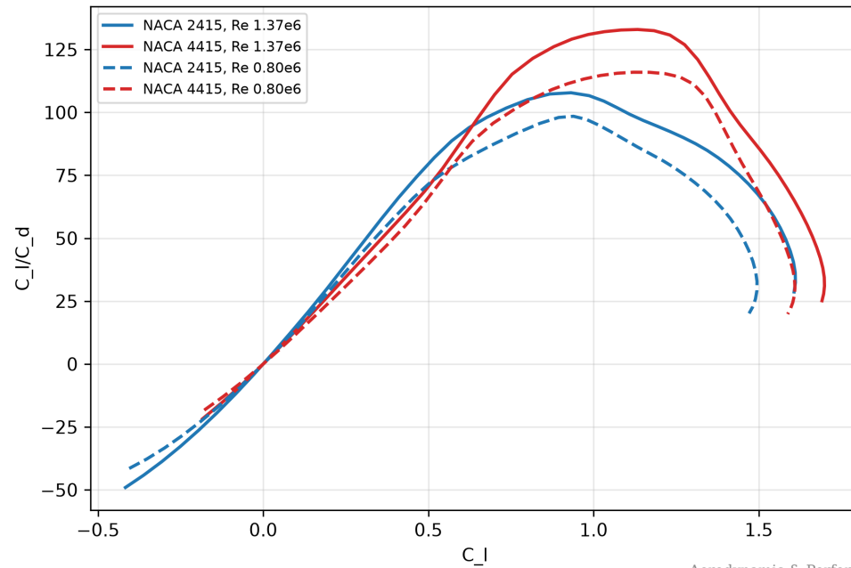
Section L/D
