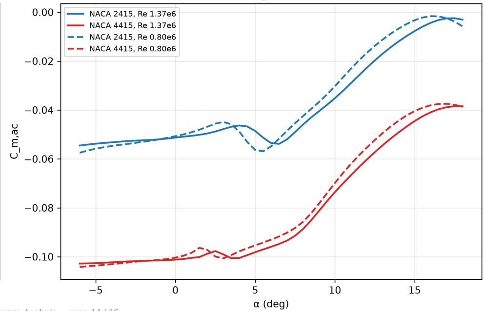
Pitching moment
