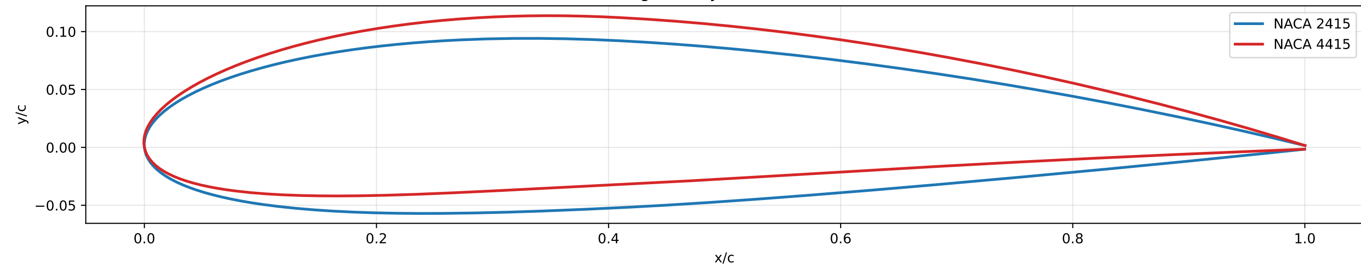
Airfoil geometry (both 15% thick)
