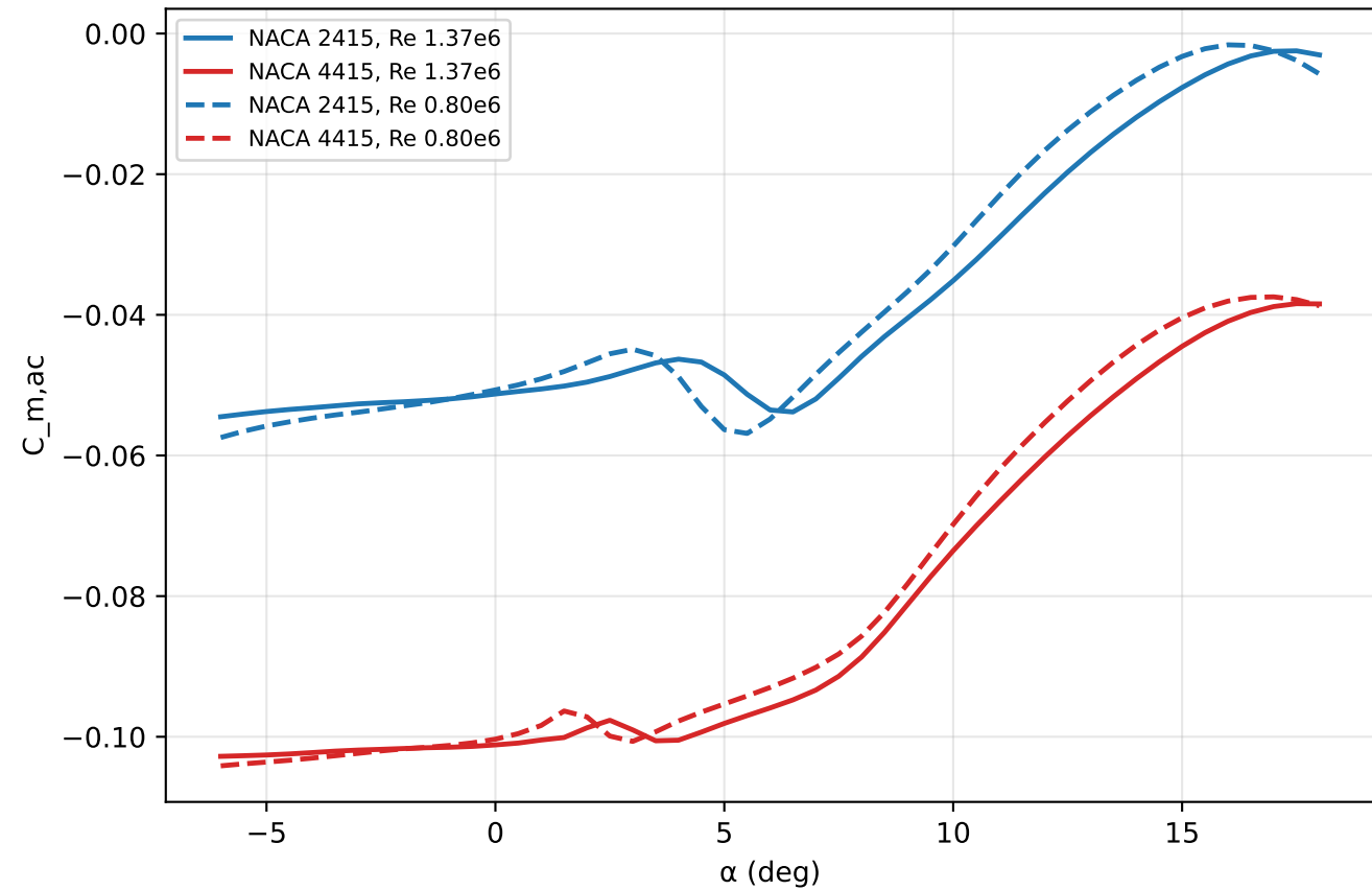
Pitching moment
