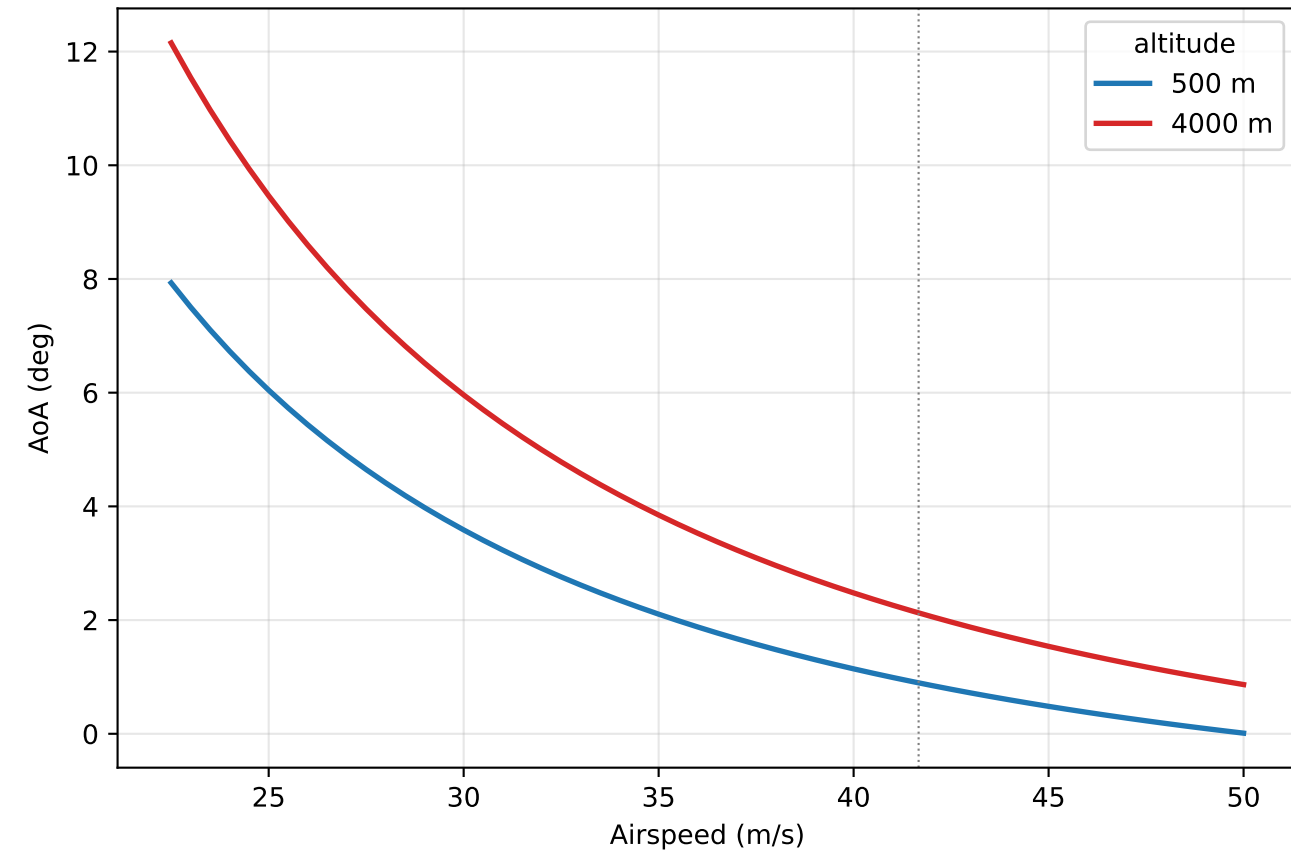
Angle of attack vs airspeed
