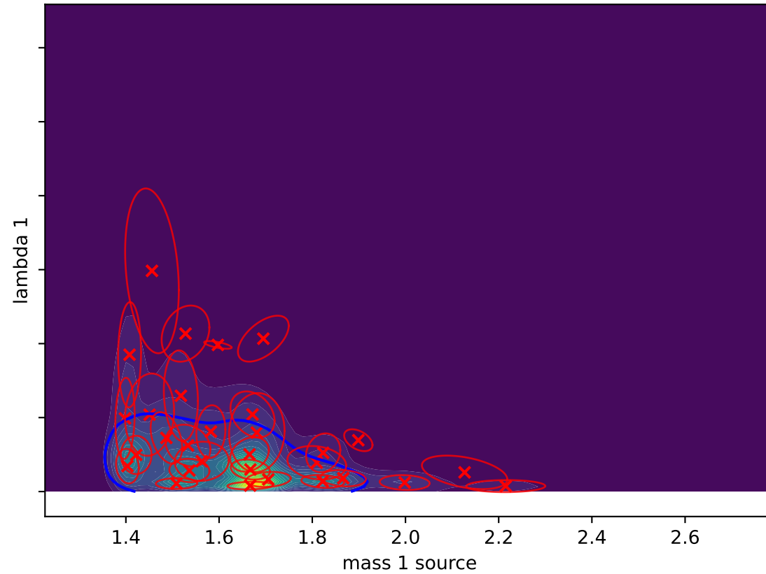
Gaussian Splat (L-BFGS) D_{KL}(P||Q) = -0.0964
