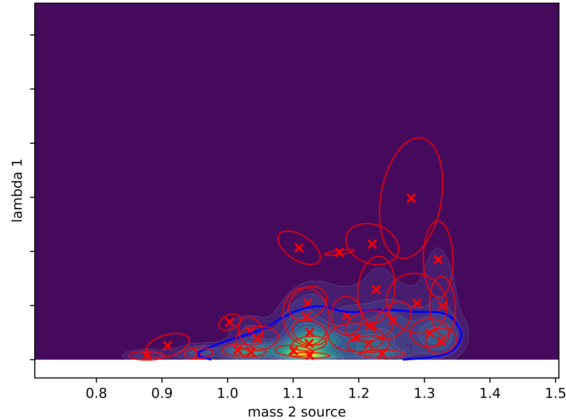
Gaussian Splat (L-BFGS) D_{KL}(P||Q) = -0.0793
