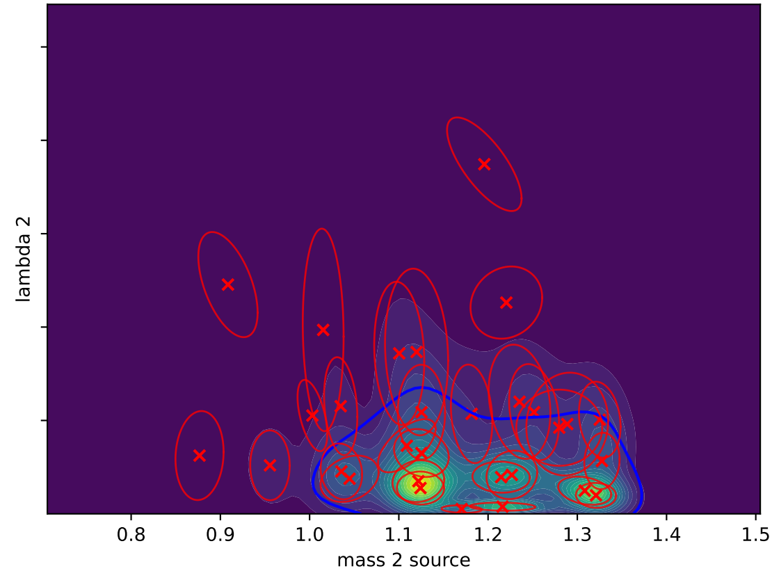
Gaussian Splat (L-BFGS) D_{KL}(P||Q) = -0.0366
