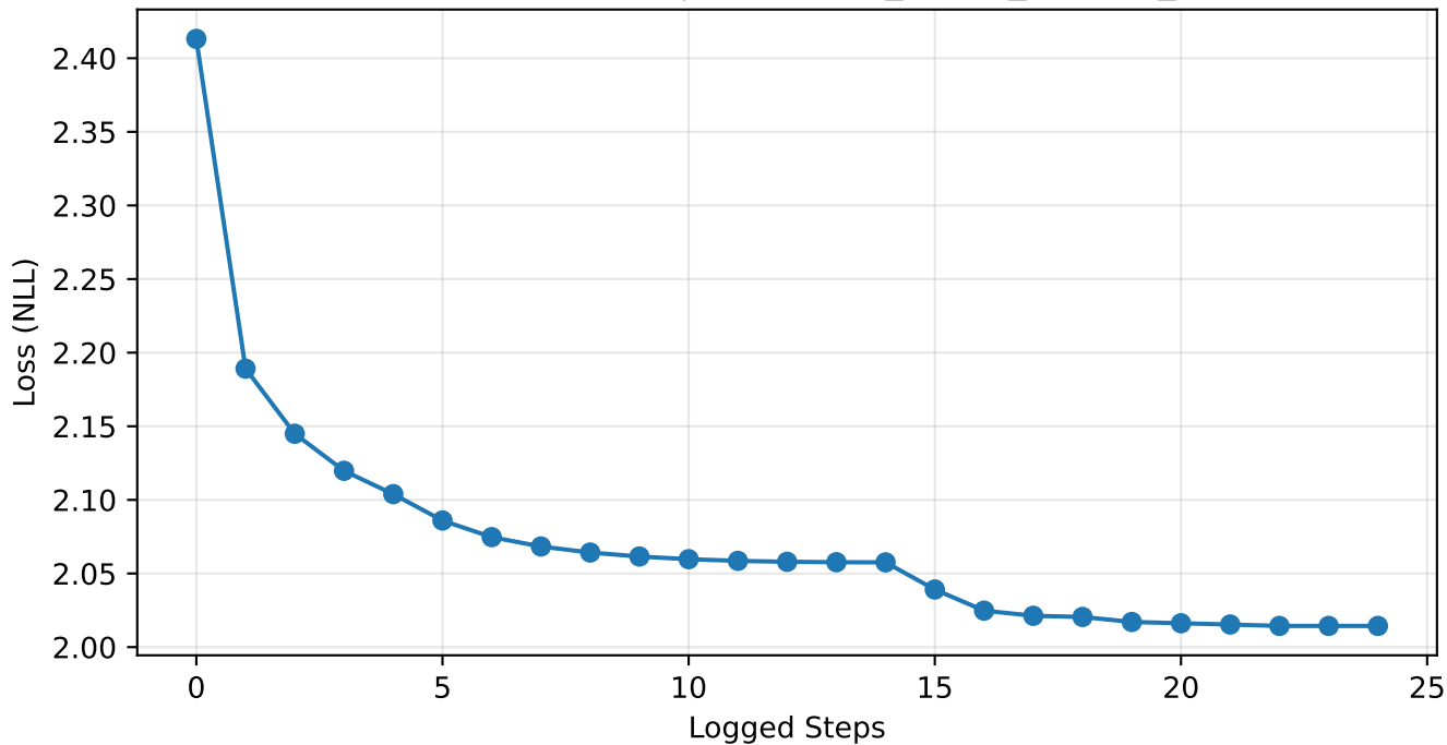
Optimization Loss Curve | gw170817_gwtc1_lowspin_posterior
