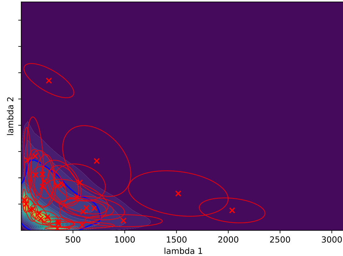
Gaussian Splat (L-BFGS) D_{KL}(P||Q) = -0.0811
