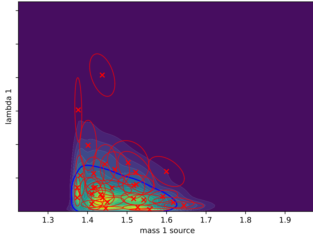
Gaussian Splat (L-BFGS) D_{KL}(P||Q) = -0.0623
