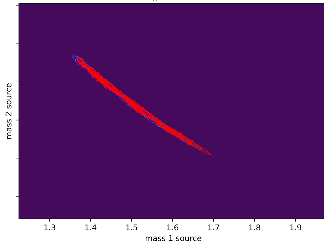
Gaussian Splat (L-BFGS) D_{KL}(P||Q) = -0.0483
