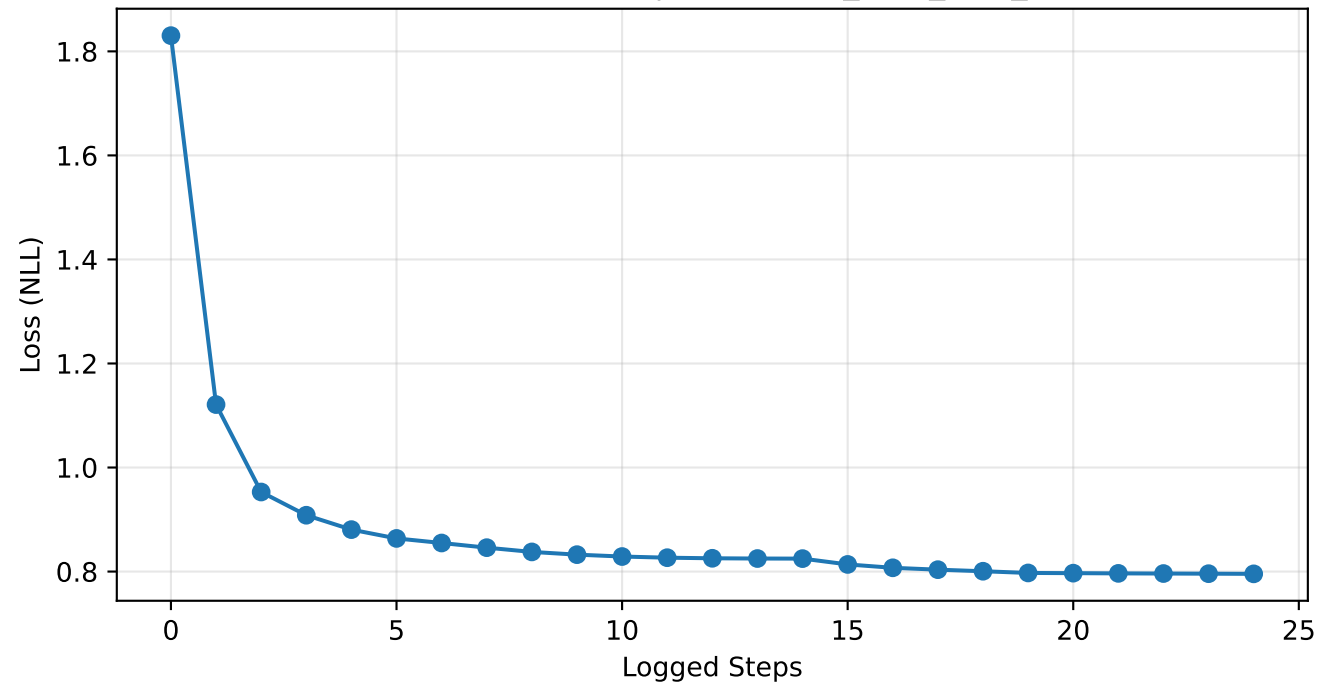
Optimization Loss Curve | gw170817_high_spin_posterior
