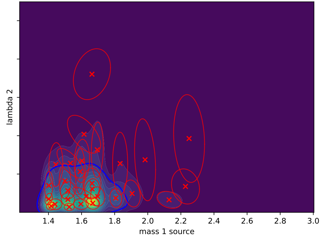
Gaussian Splat (L-BFGS) D_{KL}(P||Q) = -0.0249
