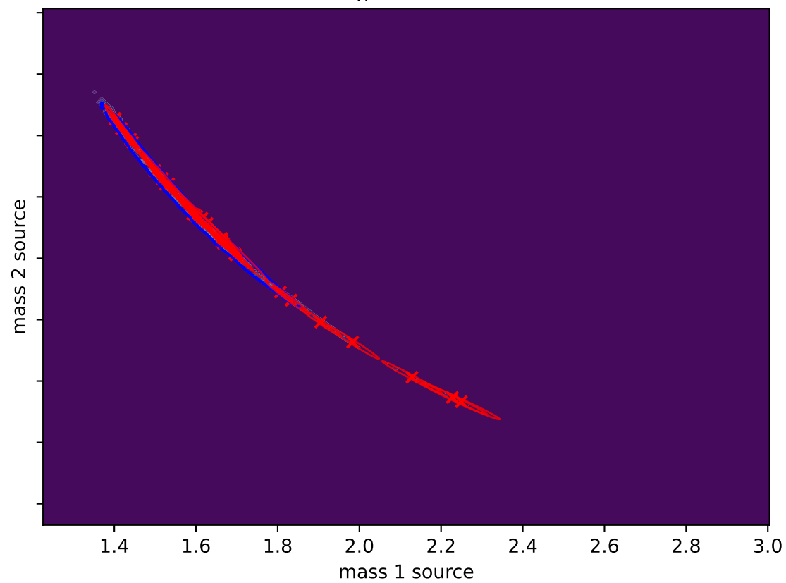
Gaussian Splat (L-BFGS) D_{KL}(P||Q) = -0.7074
