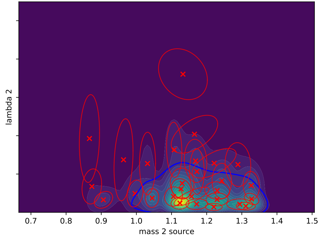
Gaussian Splat (L-BFGS) D_{KL}(P||Q) = -0.0143
