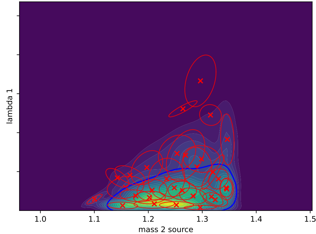
Gaussian Splat (L-BFGS) D_{KL}(P||Q) = -0.0548
