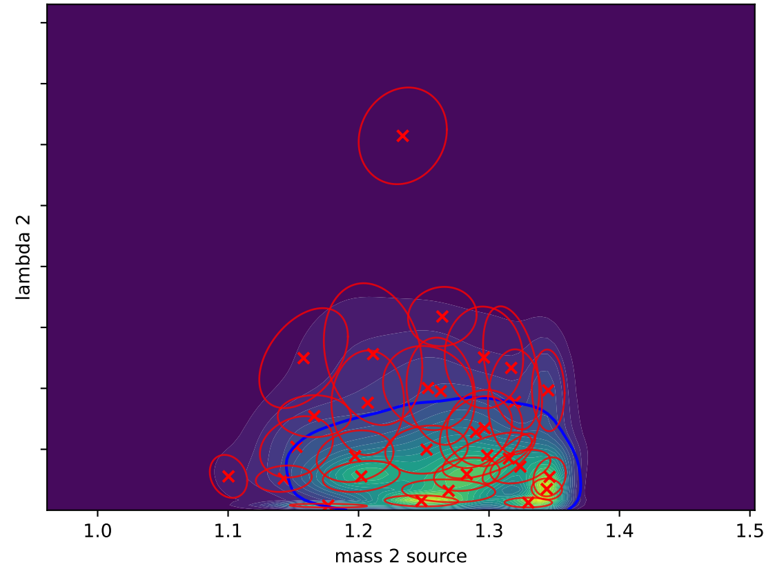
Gaussian Splat (L-BFGS) D_{KL}(P||Q) = -0.0489
