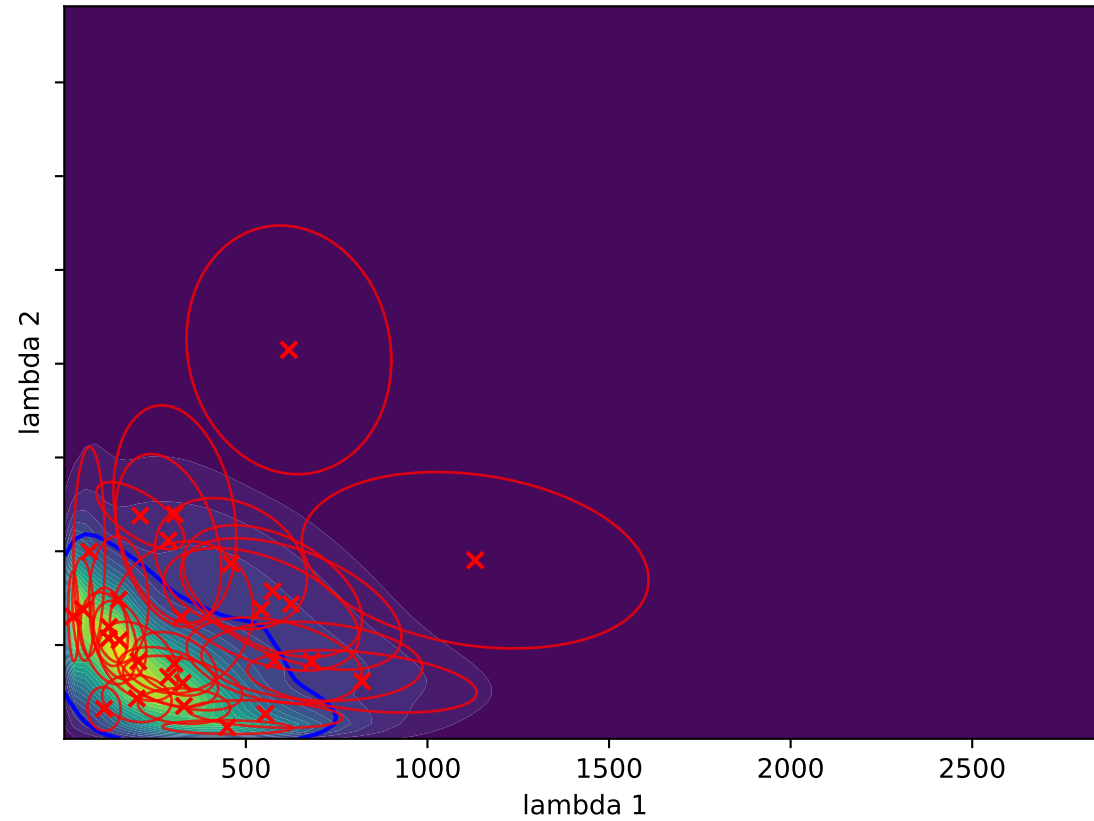
Gaussian Splat (L-BFGS) D_{KL}(P||Q) = -0.0234
