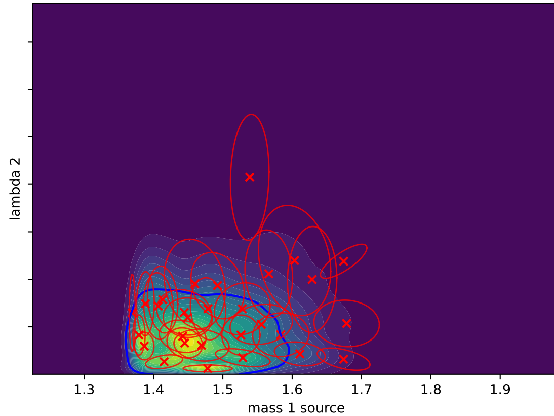
Gaussian Splat (L-BFGS) D_{KL}(P||Q) = 0.0057
