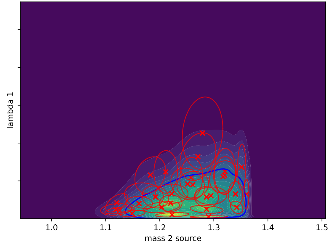
Gaussian Splat (L-BFGS) D_{KL}(P||Q) = -0.0245
