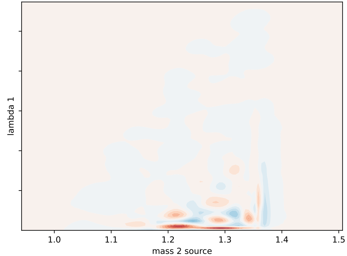
Probability Residual (P - Q)
