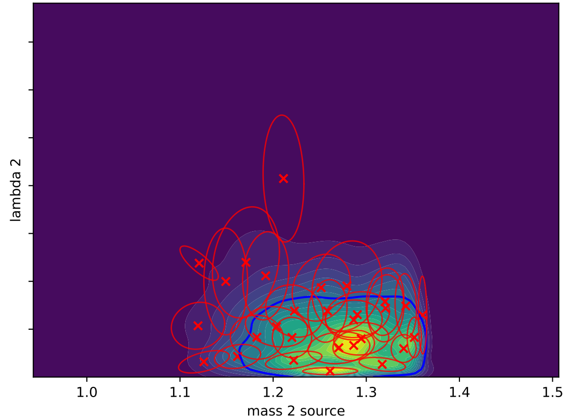
Gaussian Splat (L-BFGS) D_{KL}(P||Q) = 0.0078
