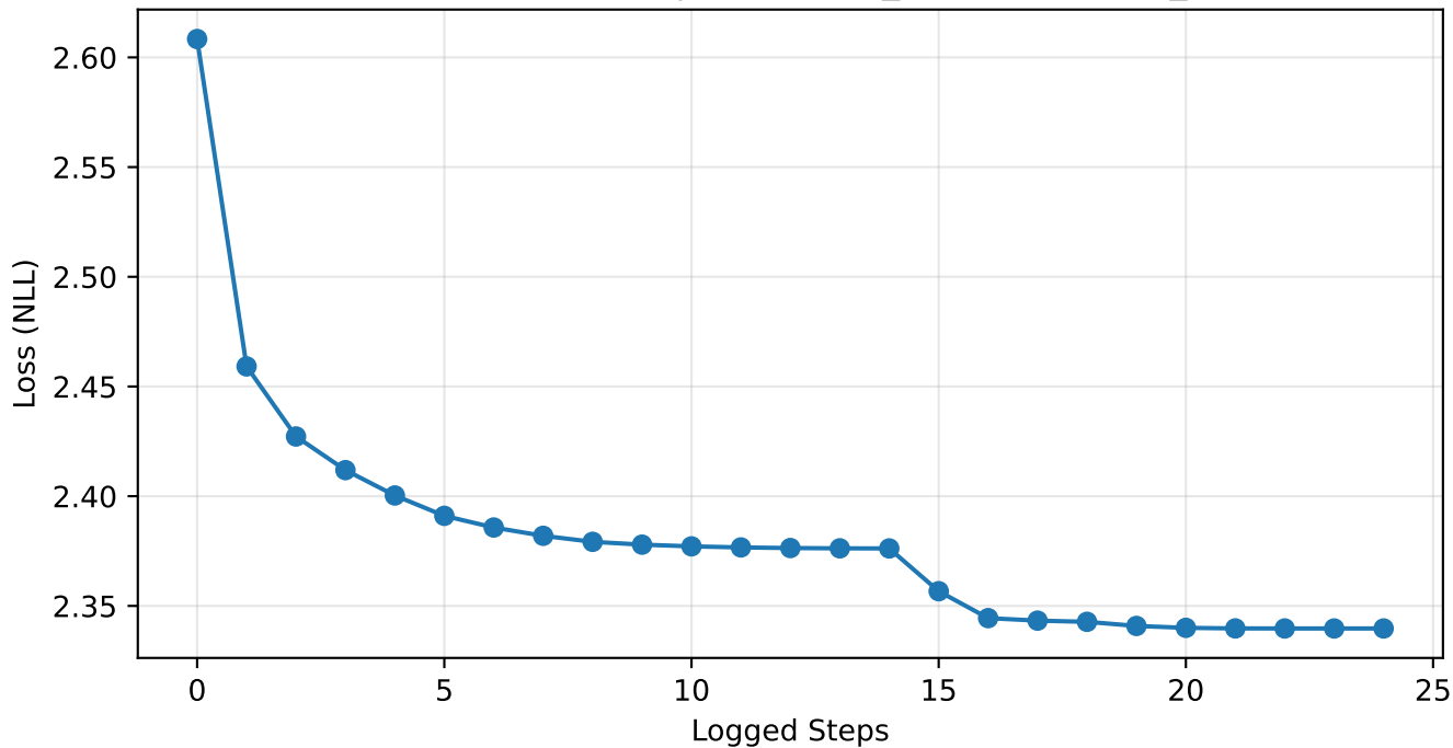
Optimization Loss Curve | gw190425_phenomdnrt-hs_posterior
