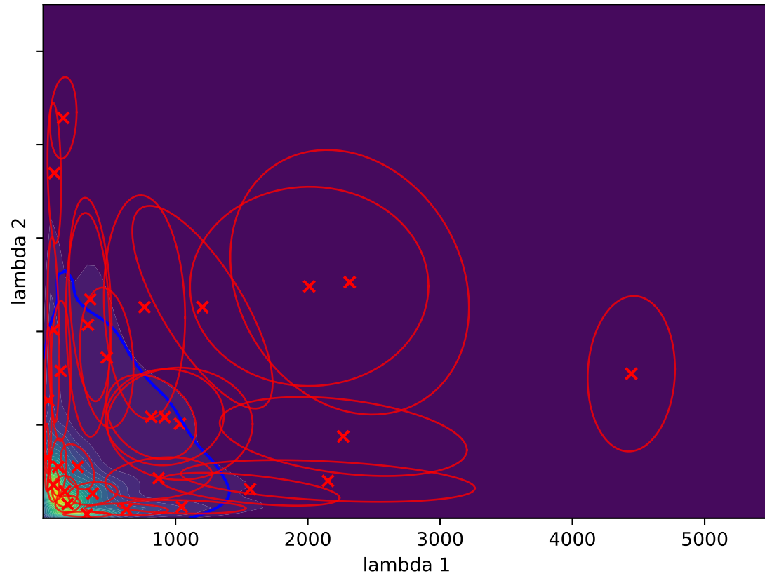
Gaussian Splat (L-BFGS) D_{KL}(P||Q) = -0.1365
