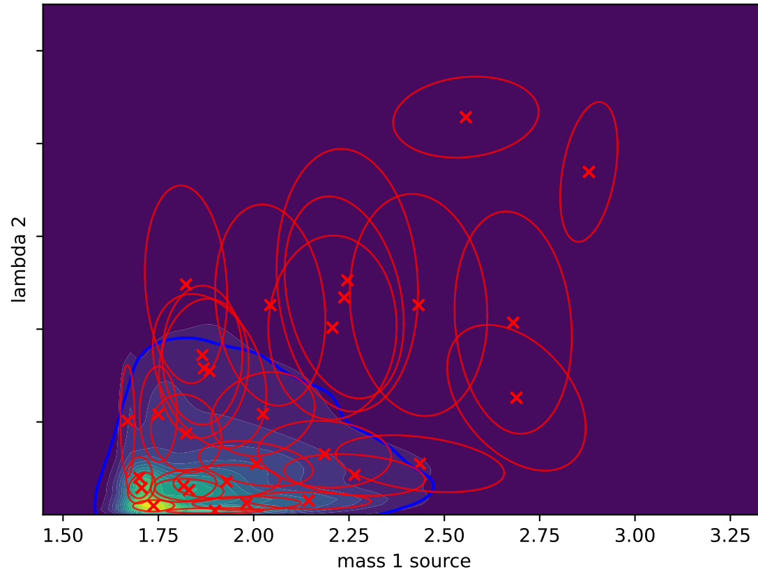
Gaussian Splat (L-BFGS) D_{KL}(P||Q) = -0.0625
