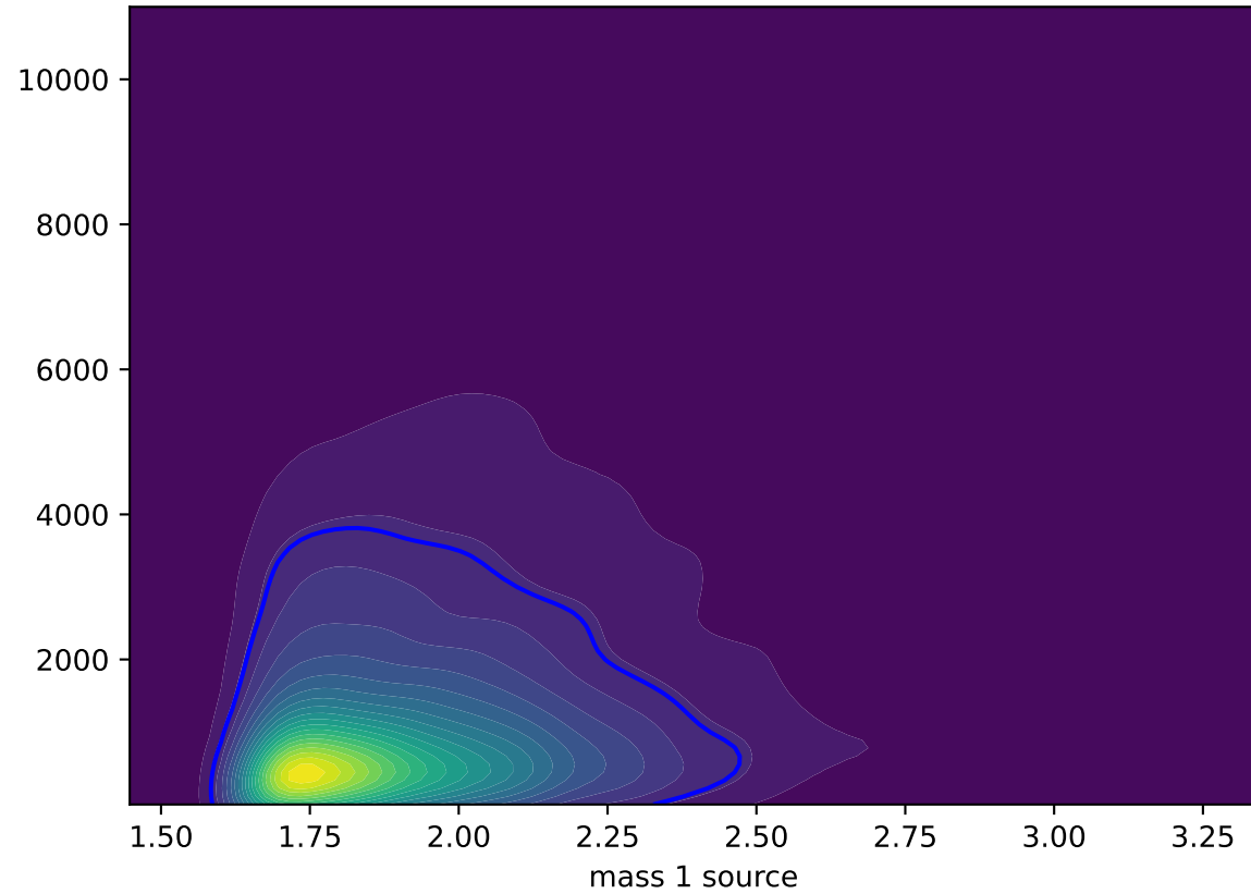
Original KDE (mass 1 source vs lambda 2)
