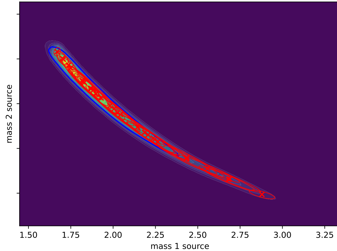
Gaussian Splat (L-BFGS) D_{\text{KL}}(P||Q) = -0.0129
