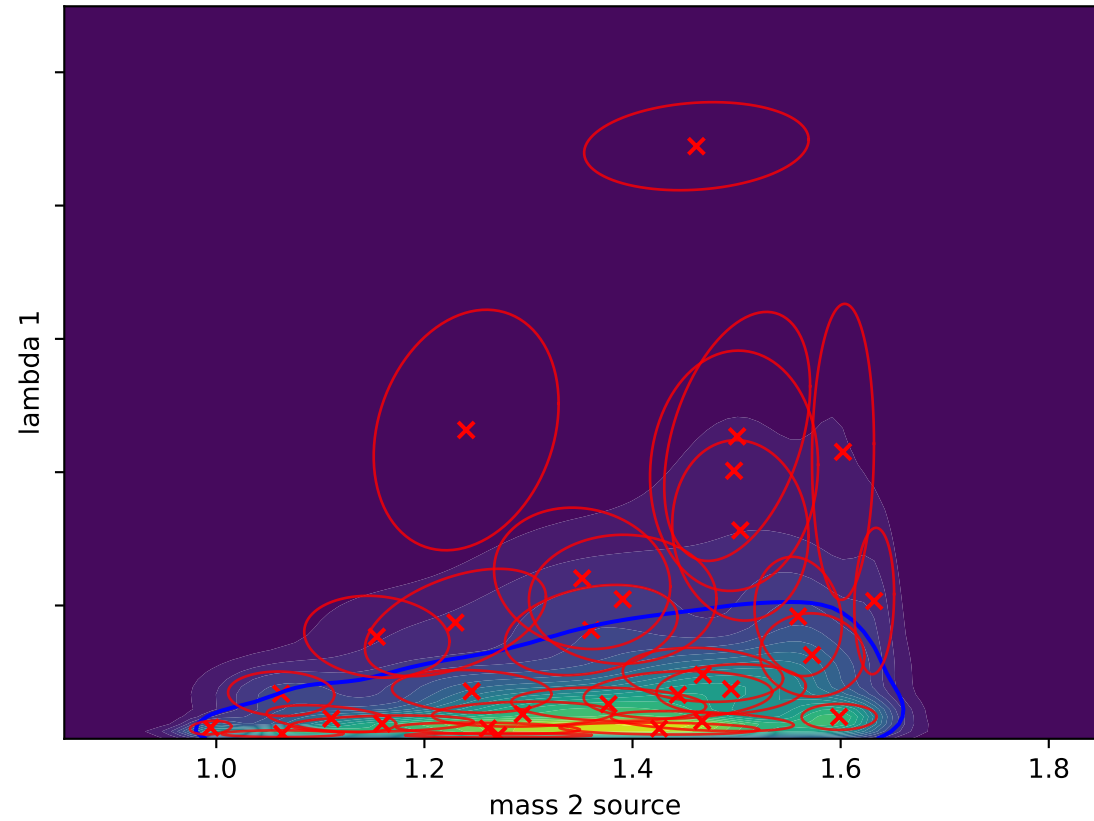
Gaussian Splat (L-BFGS) D_{KL}(P||Q) = -0.0828
