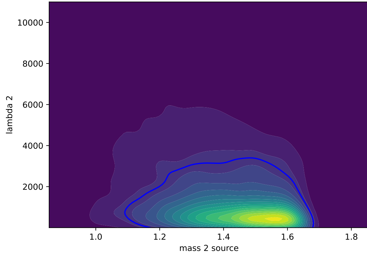
Original KDE (mass 2 source vs lambda 2)
