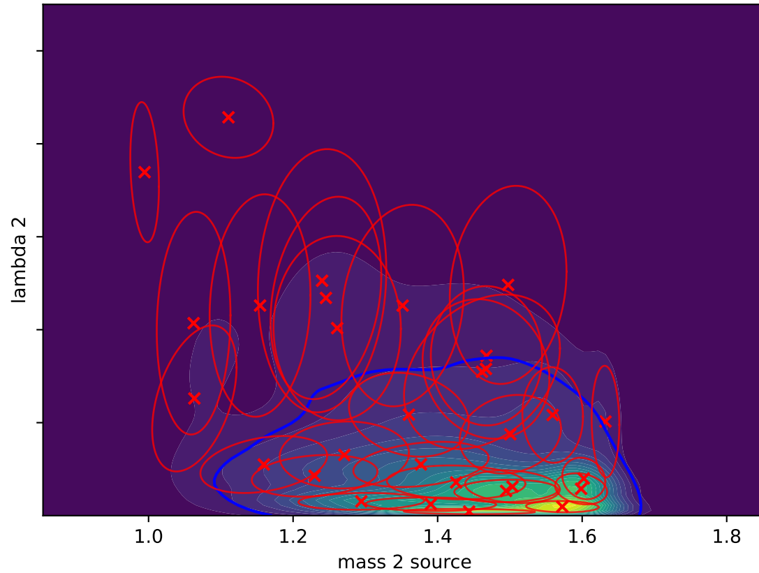
Gaussian Splat (L-BFGS) D_{KL}(P||Q) = -0.0507
