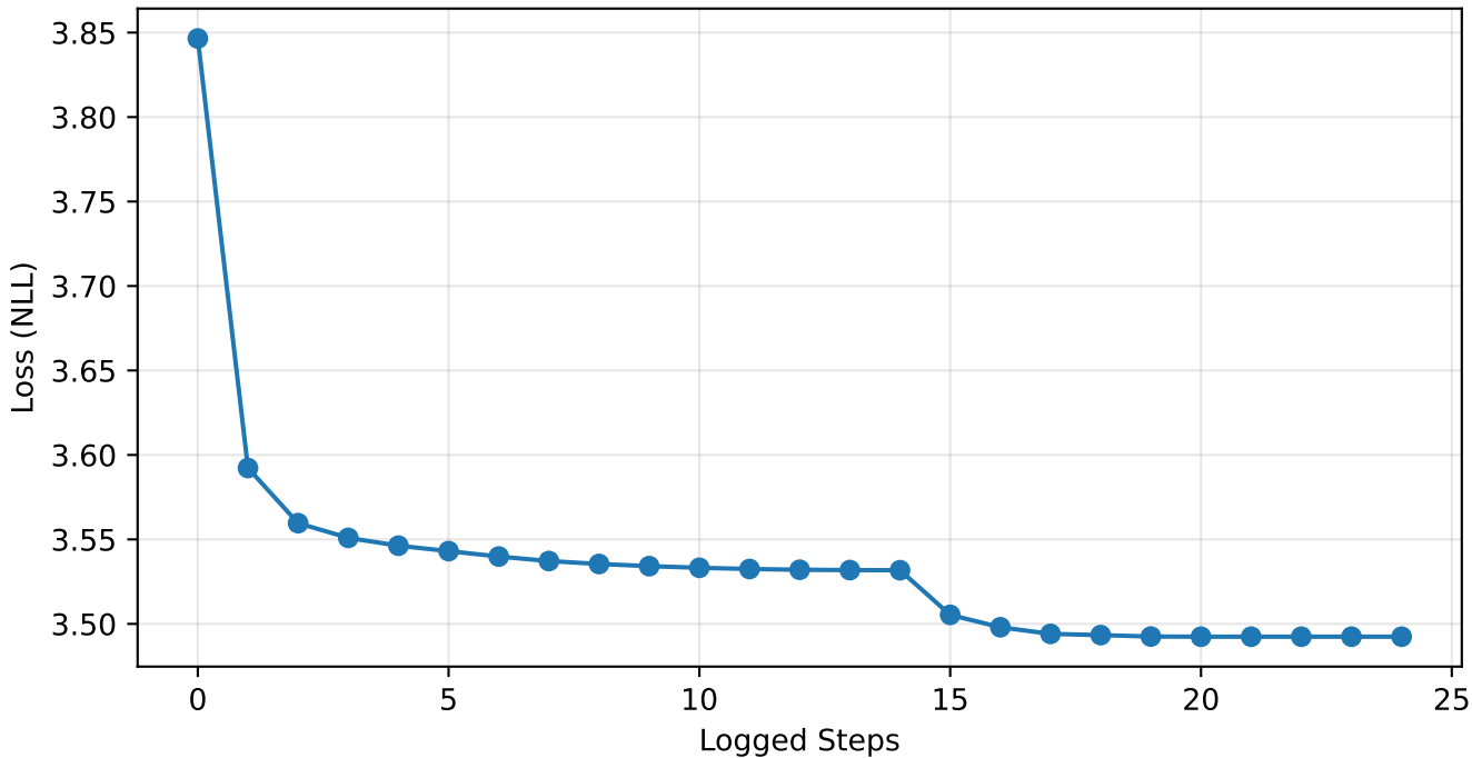
Optimization Loss Curve | gw190425_phenomdnrt-ls_posterior
