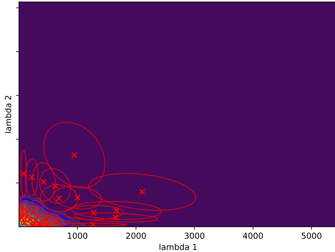
Gaussian Splat (L-BFGS) D_{KL}(P||Q) = -0.1152
