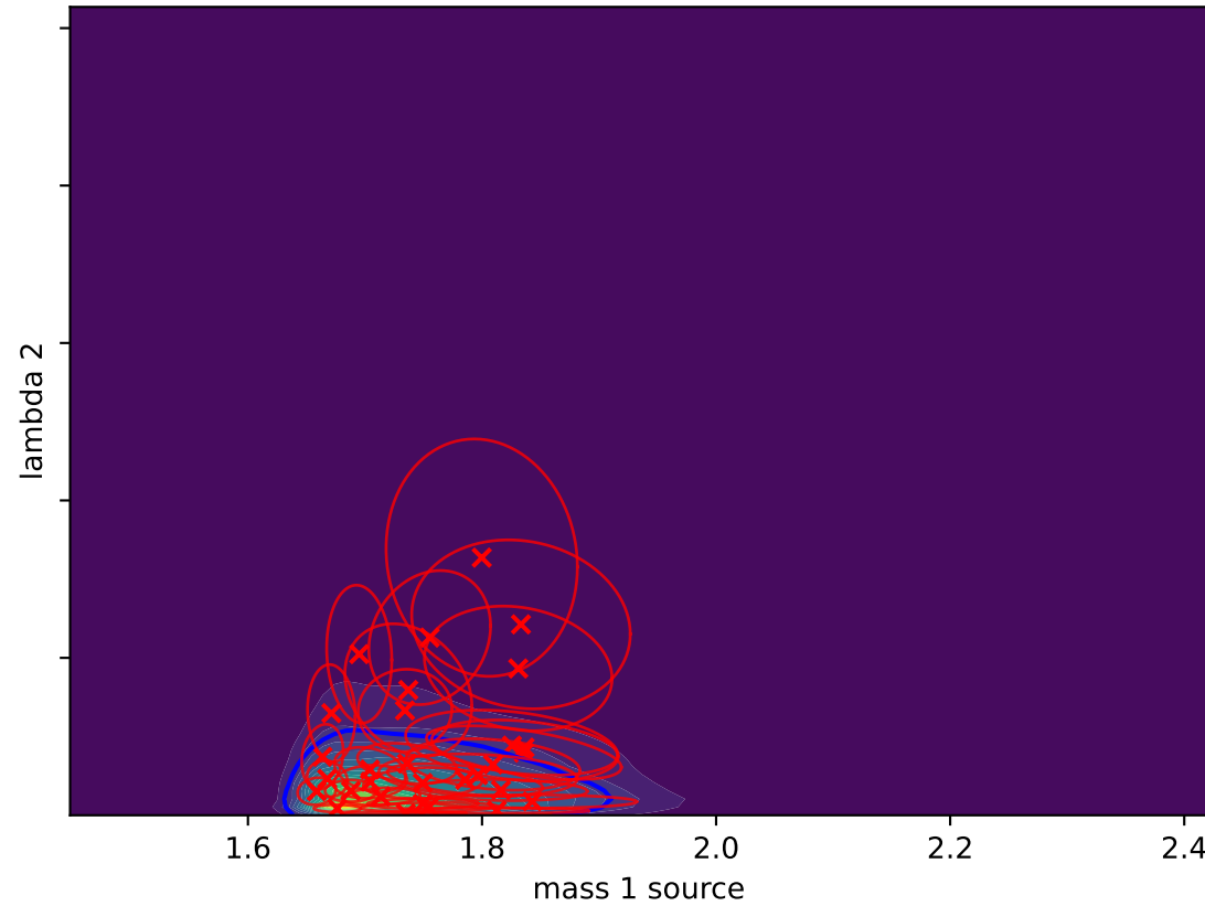
Gaussian Splat (L-BFGS) D_{KL}(P||Q) = -0.0532
