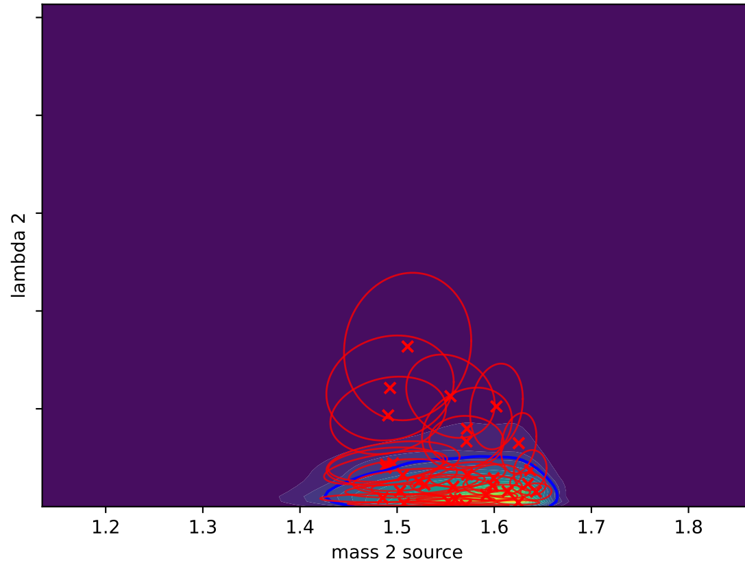
Gaussian Splat (L-BFGS) D_{KL}(P||Q) = -0.0538
