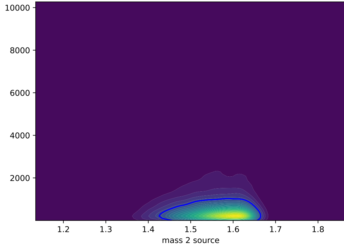
Original KDE (mass 2 source vs lambda 2)
